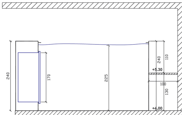
section 1-1
